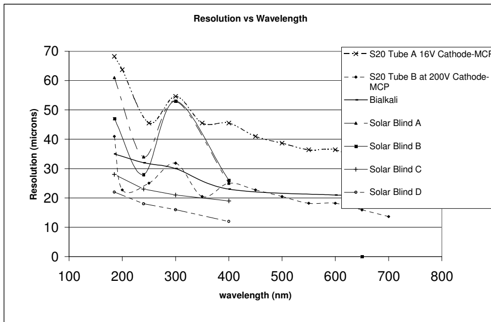
Figure 6 Resolution measurements as a function of wavelength for different tubes.
