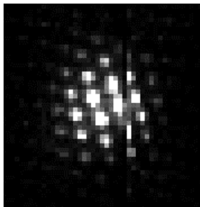
Figure (2) Centroided image of projected spot at x32 pixel binning. The hexagonal structure of the MCP pores can clearly be seen. In this example the pores are 12 microns in diameter and 15 microns from centre to centre.
