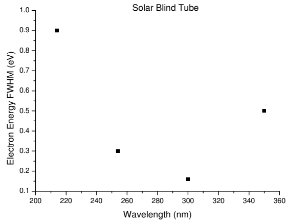
Figure 9 Electron energy FWHM plotted as a function of wavelength – Solar Blind Tube
