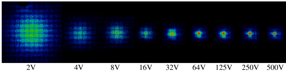
Figure (4) Solar blind image intensifier tube running at 185 nm, 0.21 mm cathode-MCP gap (note the grid pattern superimposed on the images is an artefact of the centroiding algorithm)
