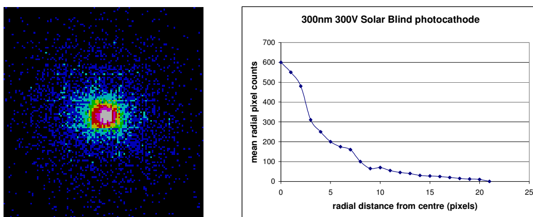
Figure (3) Centroided image of projected spot and graph showing line profile through the centre of the image
