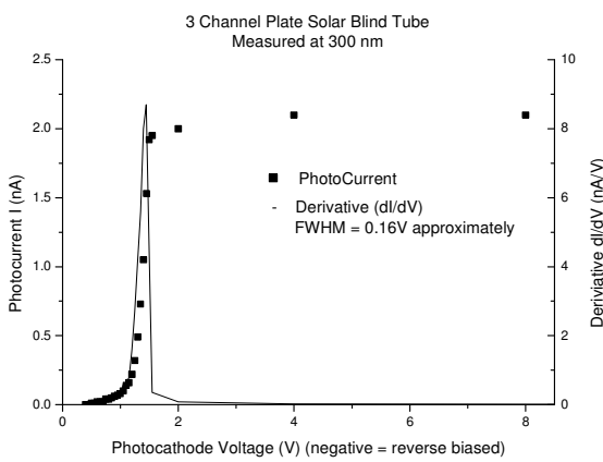
Figure 7: Electron Energy Distribution plots and \frac{dI}{dV} plots for 3 MCP Solar Blind Tube at different wavelengths
