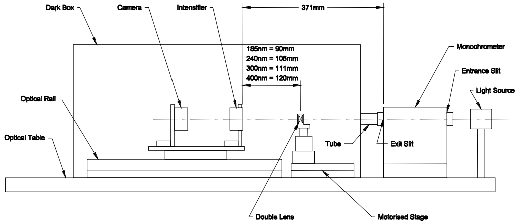
Figure (1) Diagram of resolution measurement equipment
